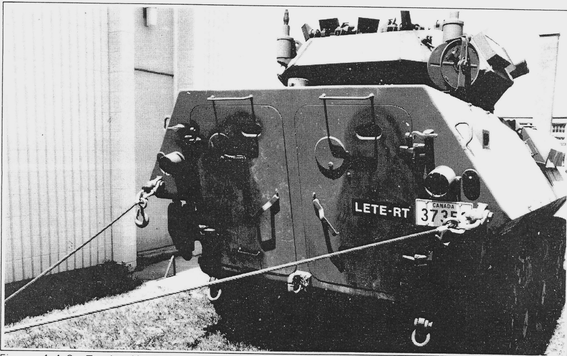
Figure 4-4-3 Towing Hook-Up — Alternate Method Raccordement de remorquage — méthode alternative
