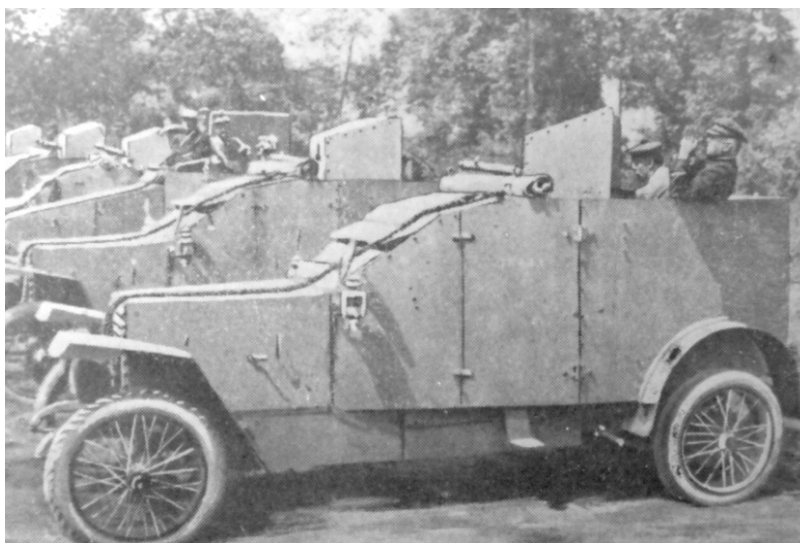
Peugeot Model 1914 type 2 armored cars. The top photo shows a Peugeot being manned by French Marines. (Photo: ECPA)
